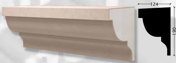
CG-25 - 190x124x1500 mm
