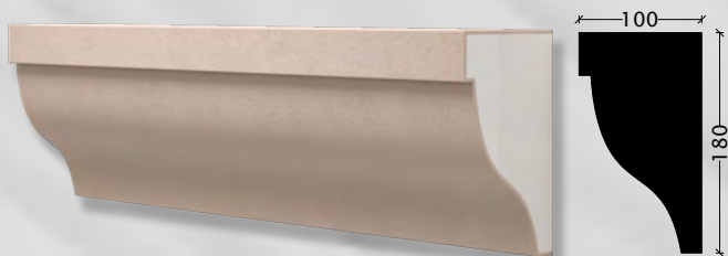
CG-29 - 180x100x1500 mm
