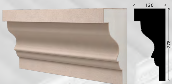
CG-75 - 278x120x1500 mm
