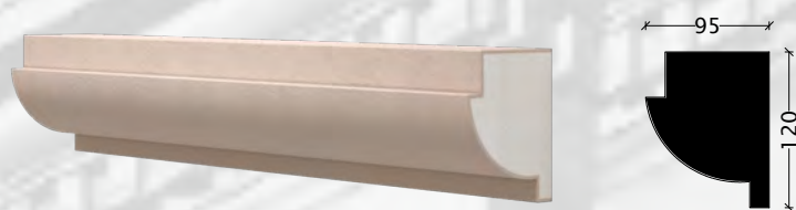
CG-67 - 120x95x1500 mm
