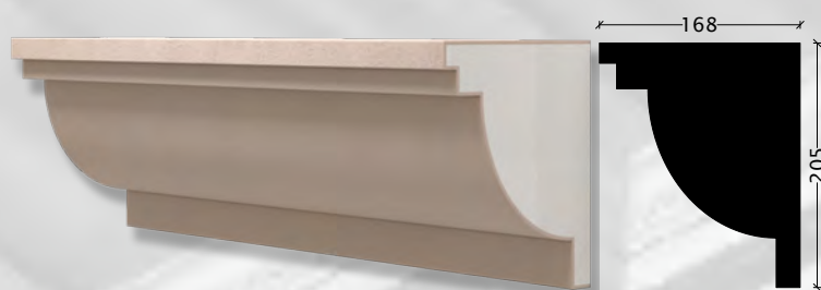
CG-55 - 205x168x1500 mm
