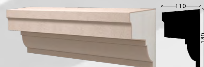
MP-49 - 180x110x1500 mm
