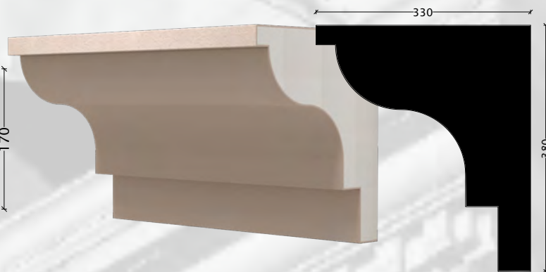
CG-62 - 380x330x1500 mm
