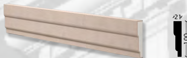
CF-138 - 100x21x1500 mm
