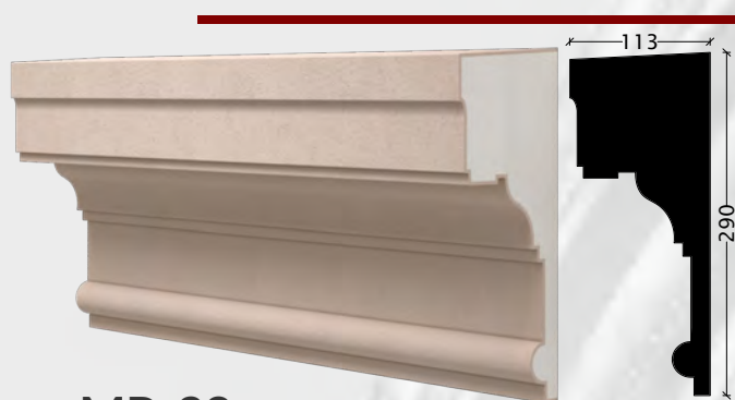
MP-38 - 290x113x1500 mm
